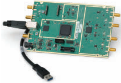
1. Model B210 is a four-channel MIMO SDR/CR with a continuous frequency range of 70 MHz to 6 GHz in a compact enclosure. Ettus Research | NI
